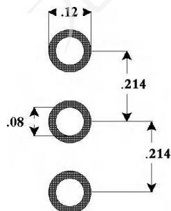
TO-247-3
